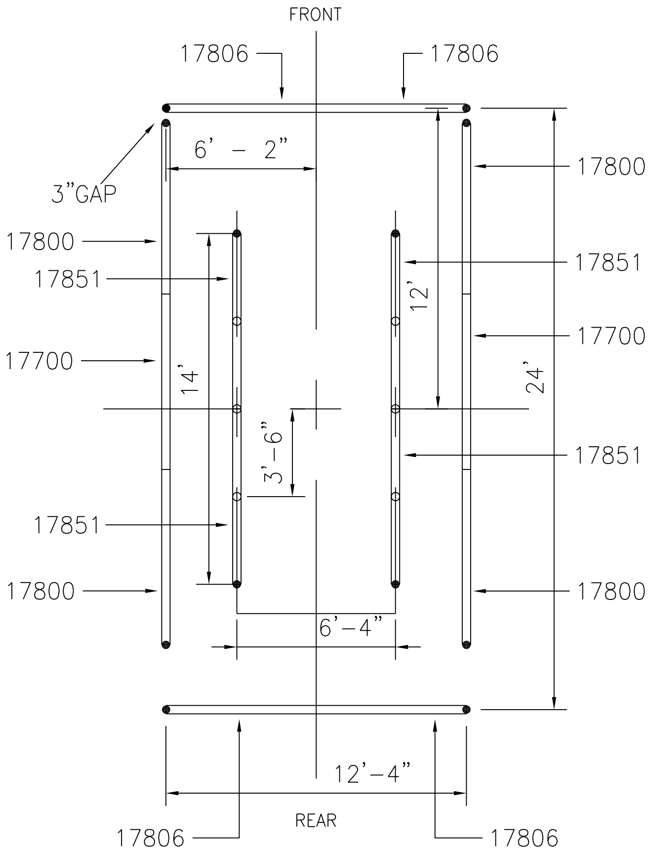
ABOVE FLOOR INSTALLATION #3 CHAINLESS ANCHORING SYSTEM WITH PULLING RAILS, MONOCOQUE TOWER & RAIL DOWN PULL
